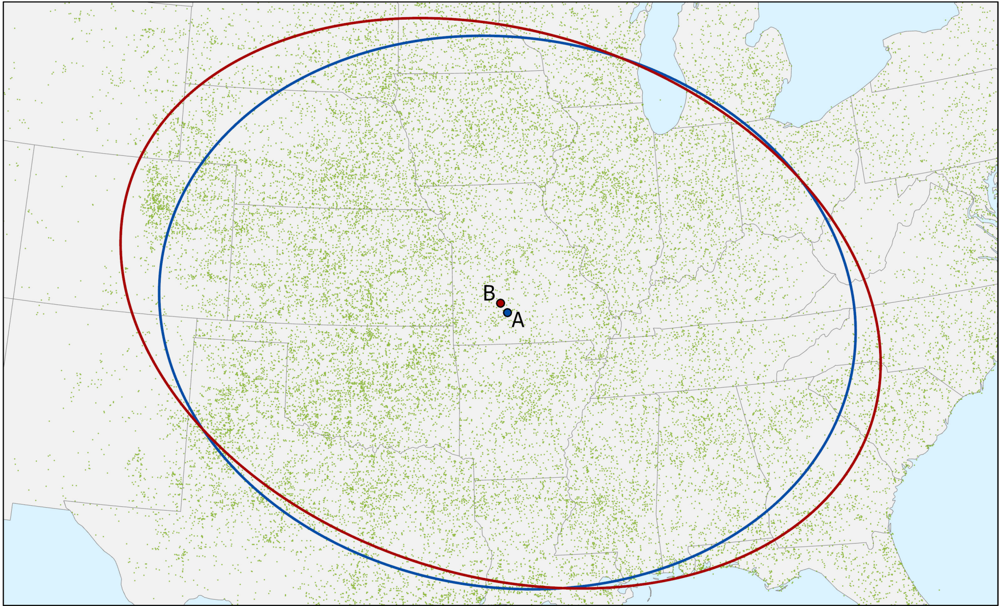
This map explores the spatial patterns in tornadoes over two time periods: A (1951-1975) and B (1981-2005). It shows standard deviational ellipses for touchdown points for the two groups as well as a center point for each ellipse.
